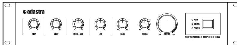
952.969 4 CHANNEL 60W RMS MIXER AMPLIFIER
